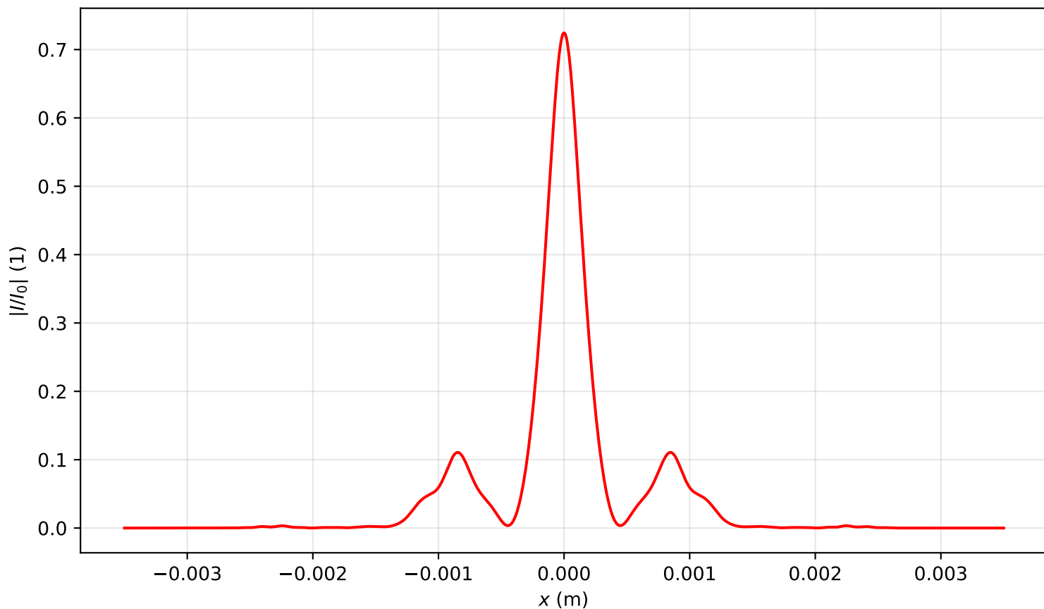
Intensity profile I(x, y = 0, z = 1.672)/I_0 , P_{in}=9.0P_{cr} , artificial time
